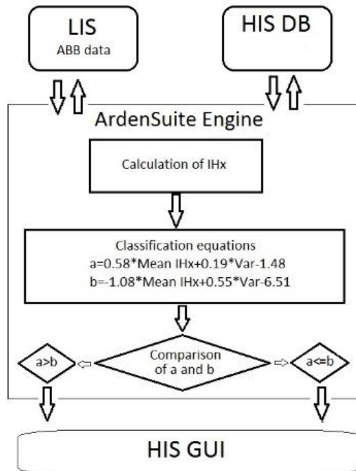
Figure 1. The IHx decision support algorithm implemented in Arden Syntax. LIS stands for the laboratory information system, HIS DB for the hospital's information system database, and HIS GUI for the hospital information system graphical user interface.
